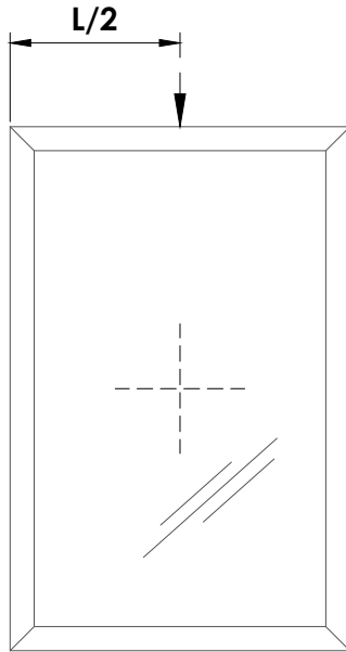
DECOMPRESSION IN FIXED WINDOW SABİT PENCEREDE BASINÇ DENGELEME
